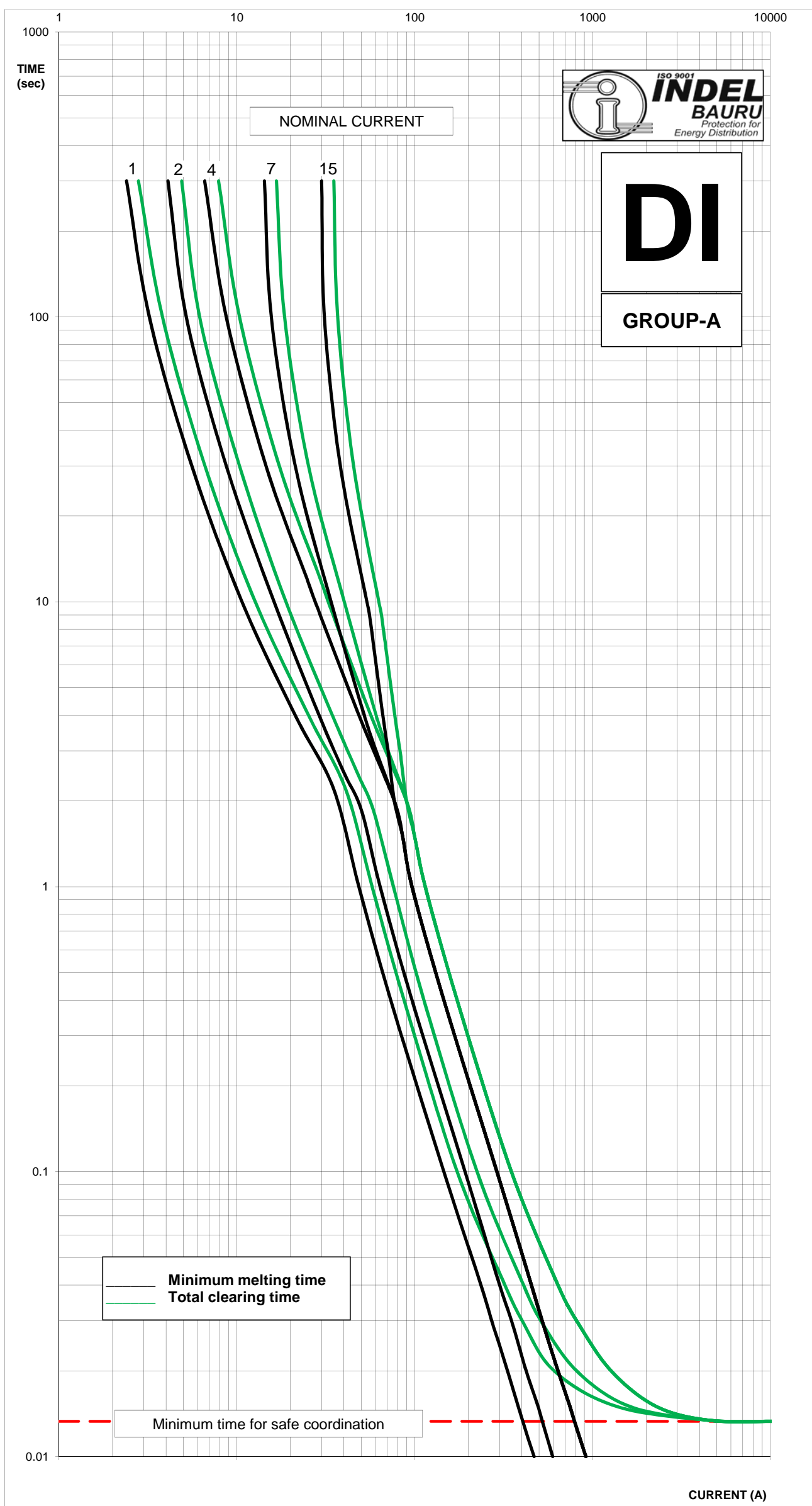
CHARACTERISTICS CURVES FUSION TIME x CURRENT TYPE "DI" - COMPLY WITH STANDARD ANSI C37.42 DATE: 08/12
