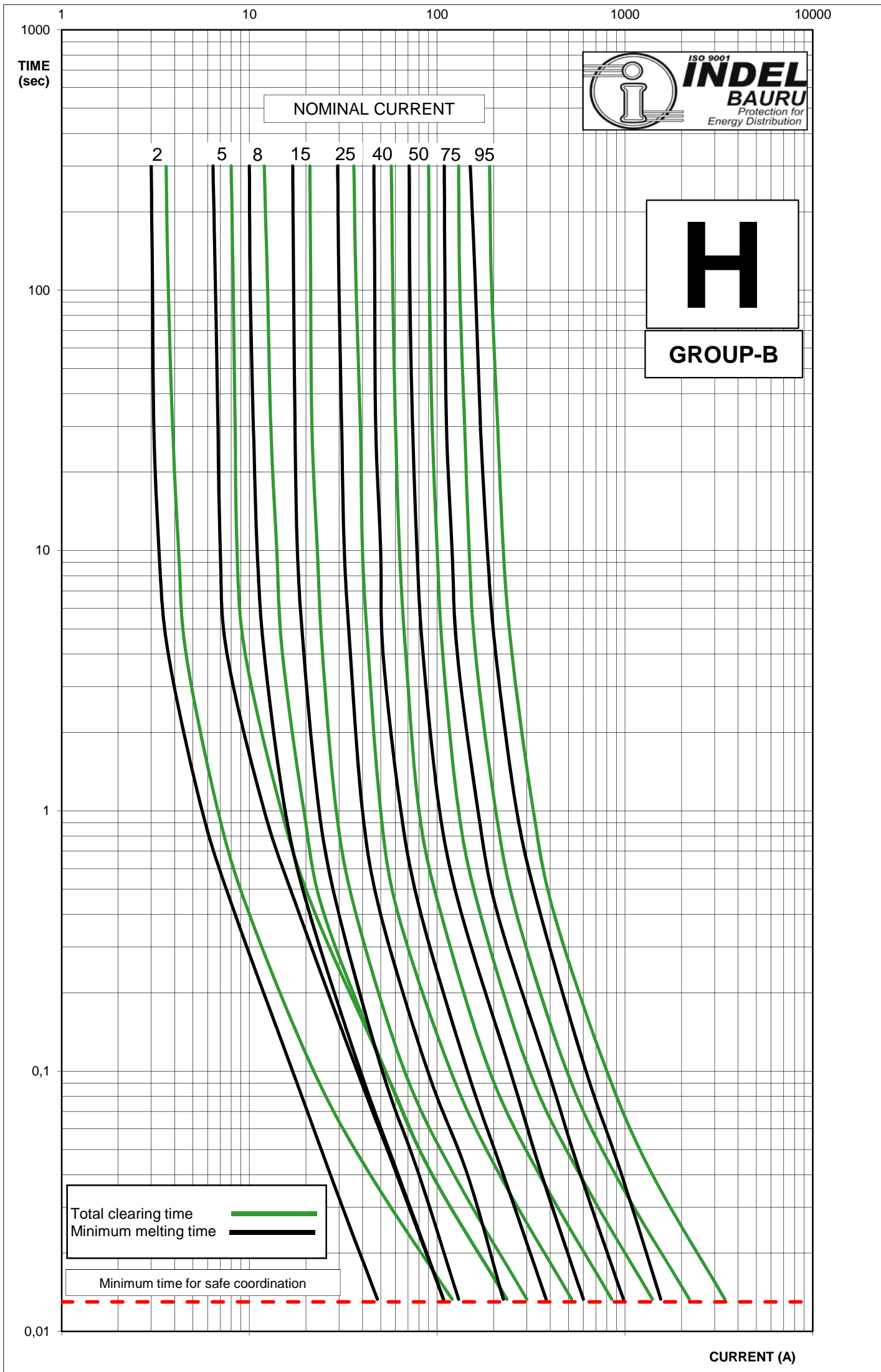
CHARACTERISTICS CURVES FUSION TIME x CURRENT TYPE "H NEMA" - COMPLY WITH STANDARD NEMA PUB SG2 DATE: 09/14
