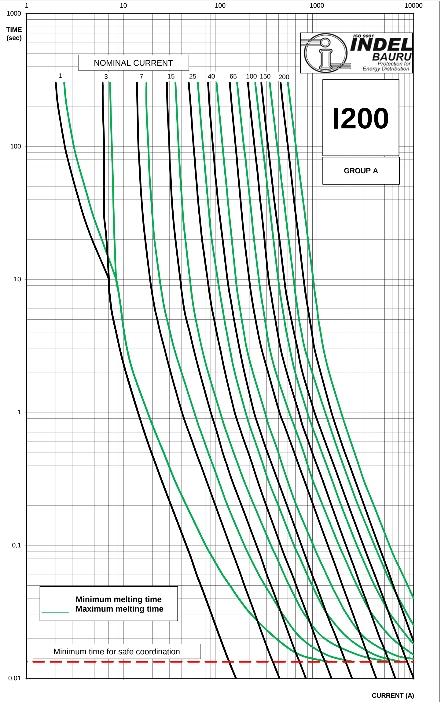
CHARACTERISTICS CURVES FUSION TIME x CURRENT TYPE "I200" - COMPLY WITH STANDARD ANSI C37.42 DATE: 02/14
