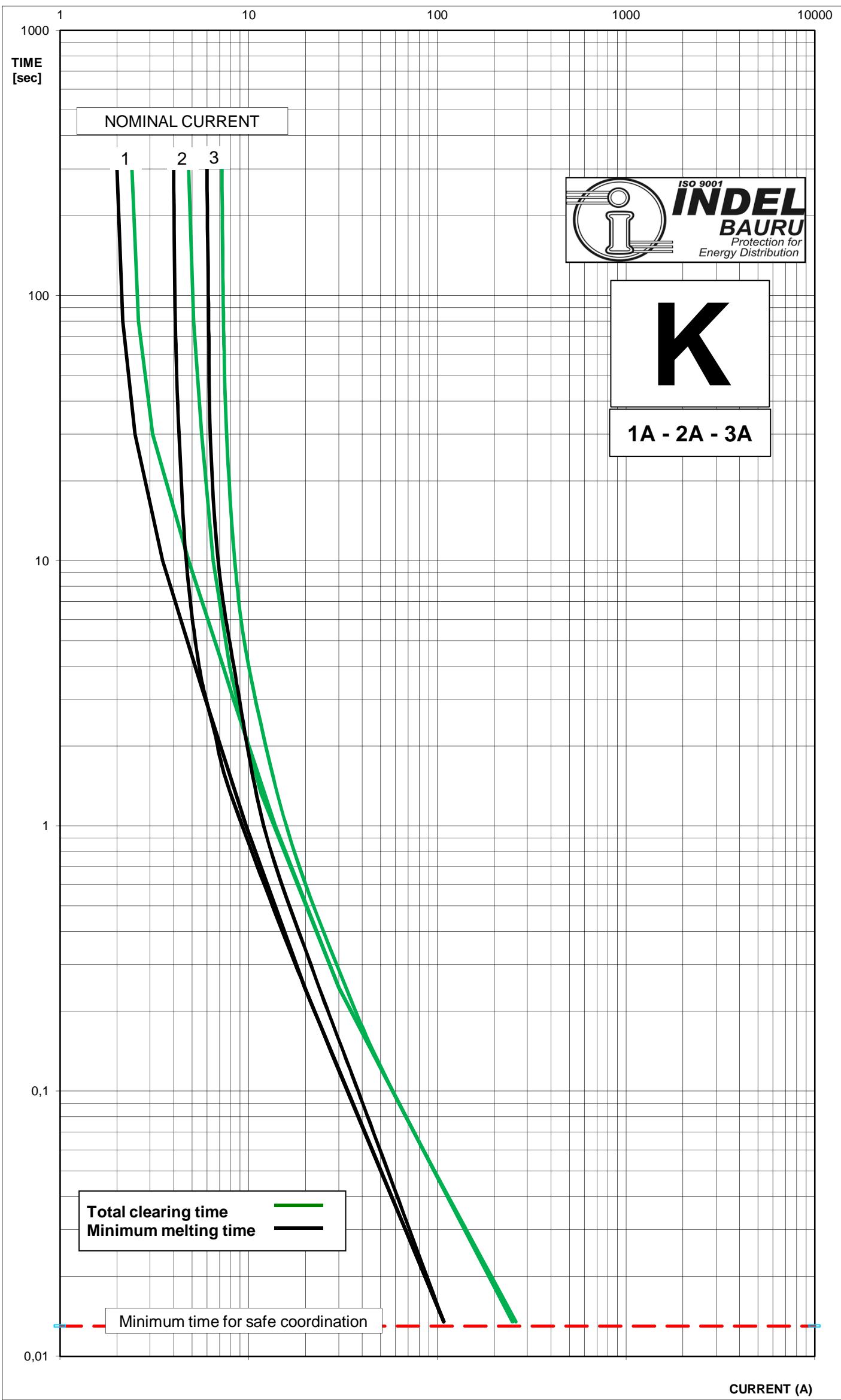
CHARACTERISTICS CURVES FUSION TIME x CURRENT TYPE "K" - COMPLY WITH STANDARD ANSI C37.42-1996 DATE: 09/02
