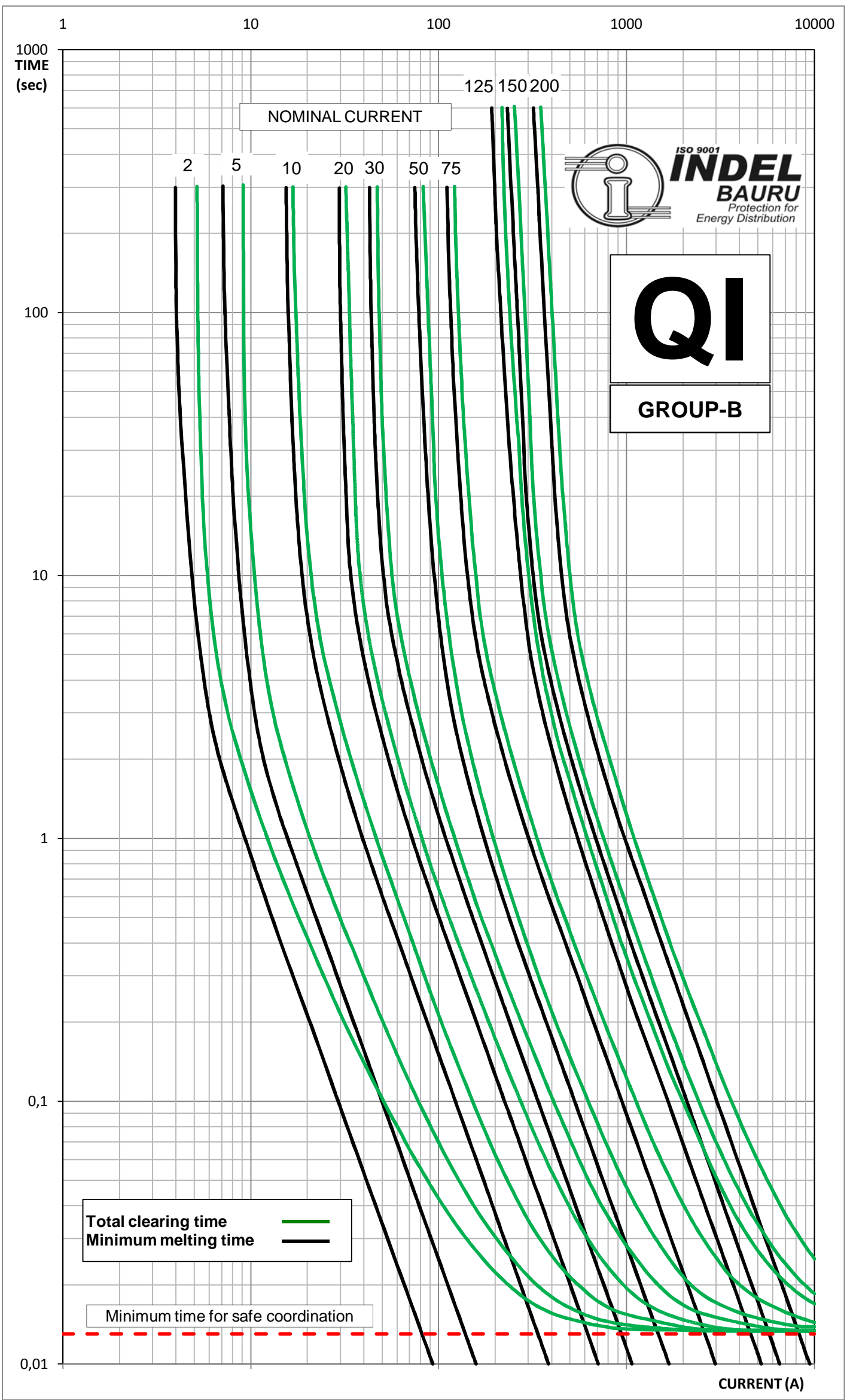
CHARACTERISTICS CURVES FUSION TIME x CURRENT TYPE "QI" - COMPLY WITH STANDARD ANSI C37.42-1996 DATE: 09/02
