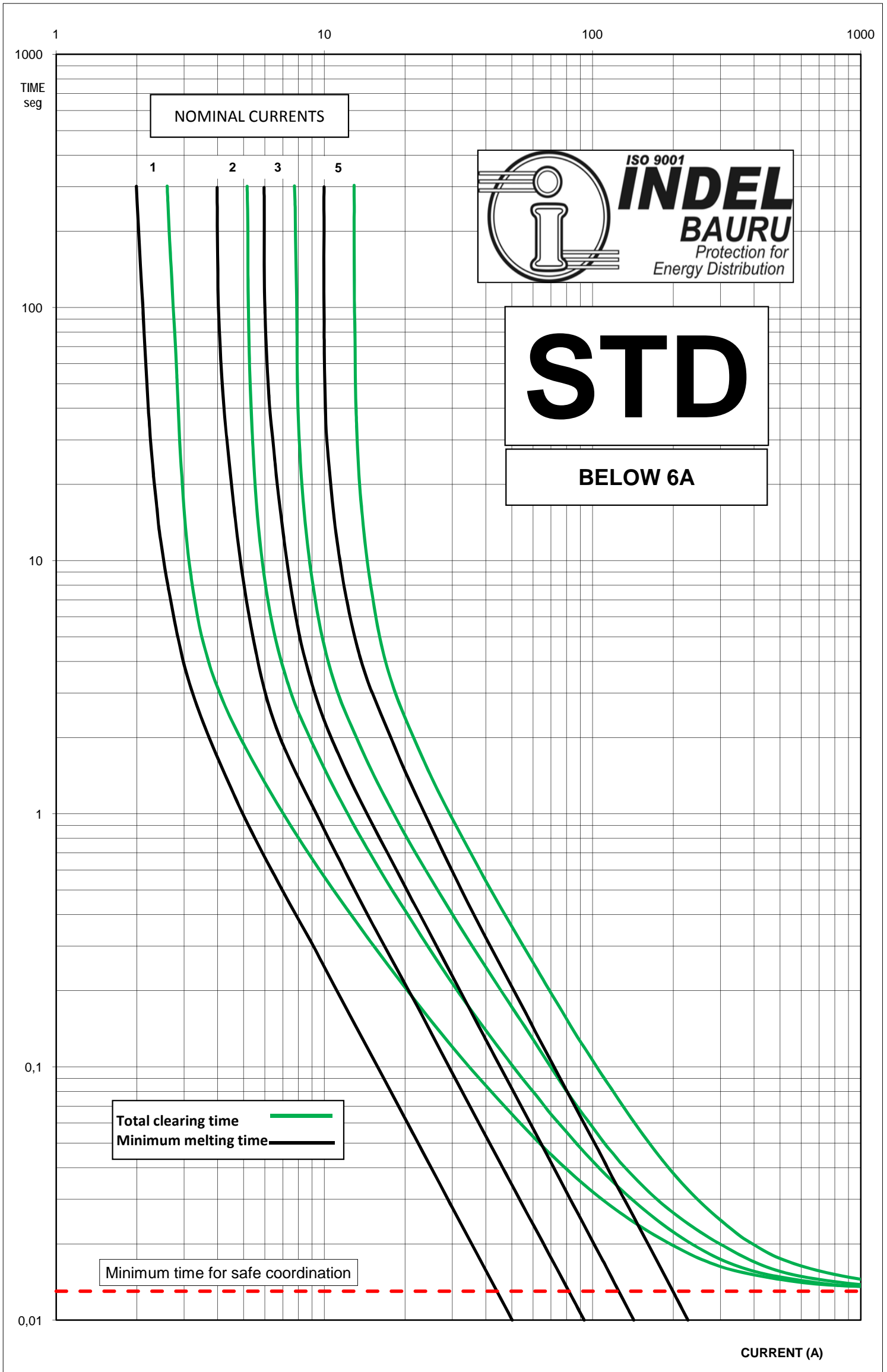
CHARACTERISTICS CURVES FUSION TIME x CURRENT TYPE "STD" - COMPLY WITH STANDARD ANSI C37.42-1996 DATE: 09/02
