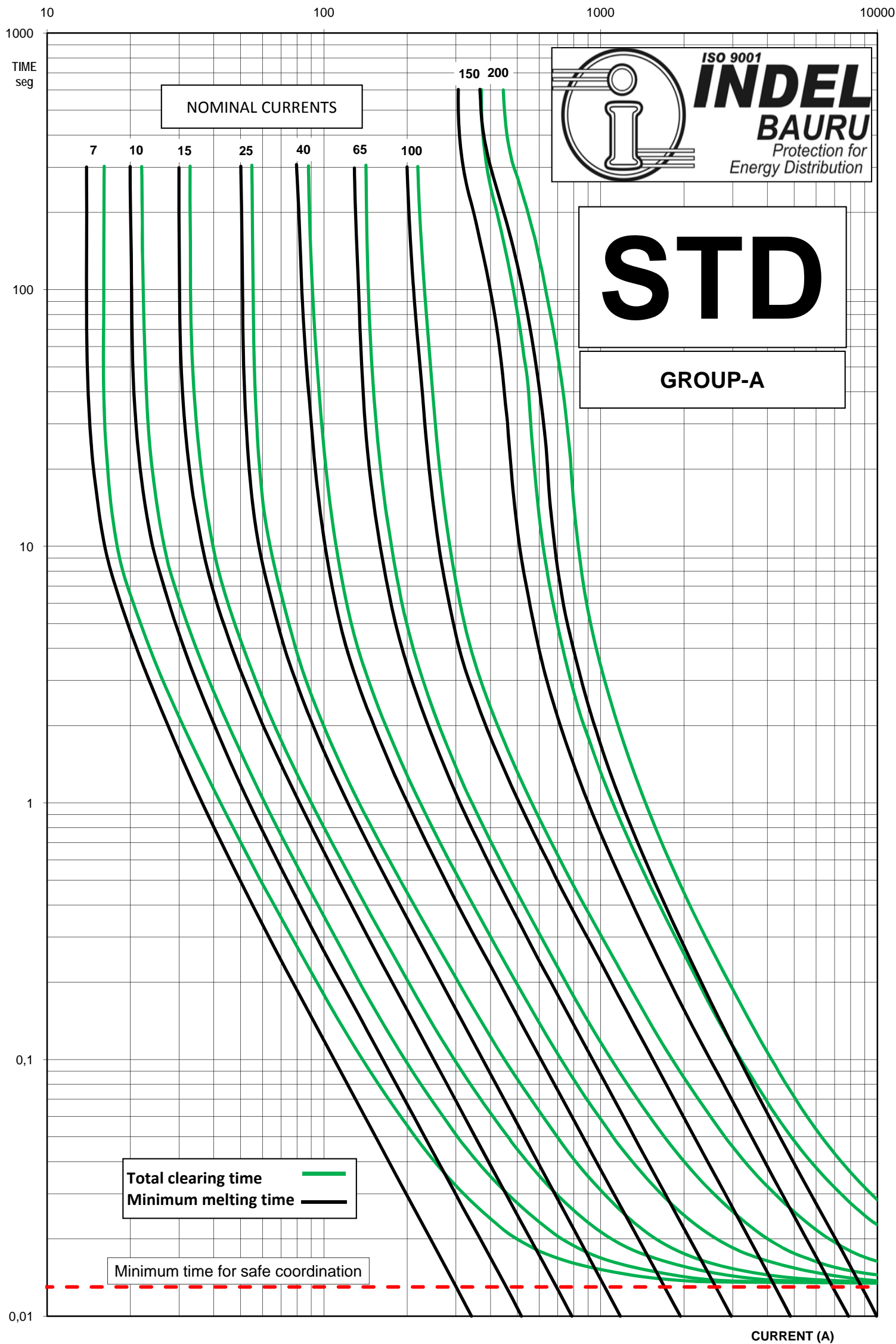
CHARACTERISTICS CURVES FUSION TIME x CURRENT TYPE "STD" - COMPLY WITH STANDARD ANSI C37.42-1996 DATE: 09/02
