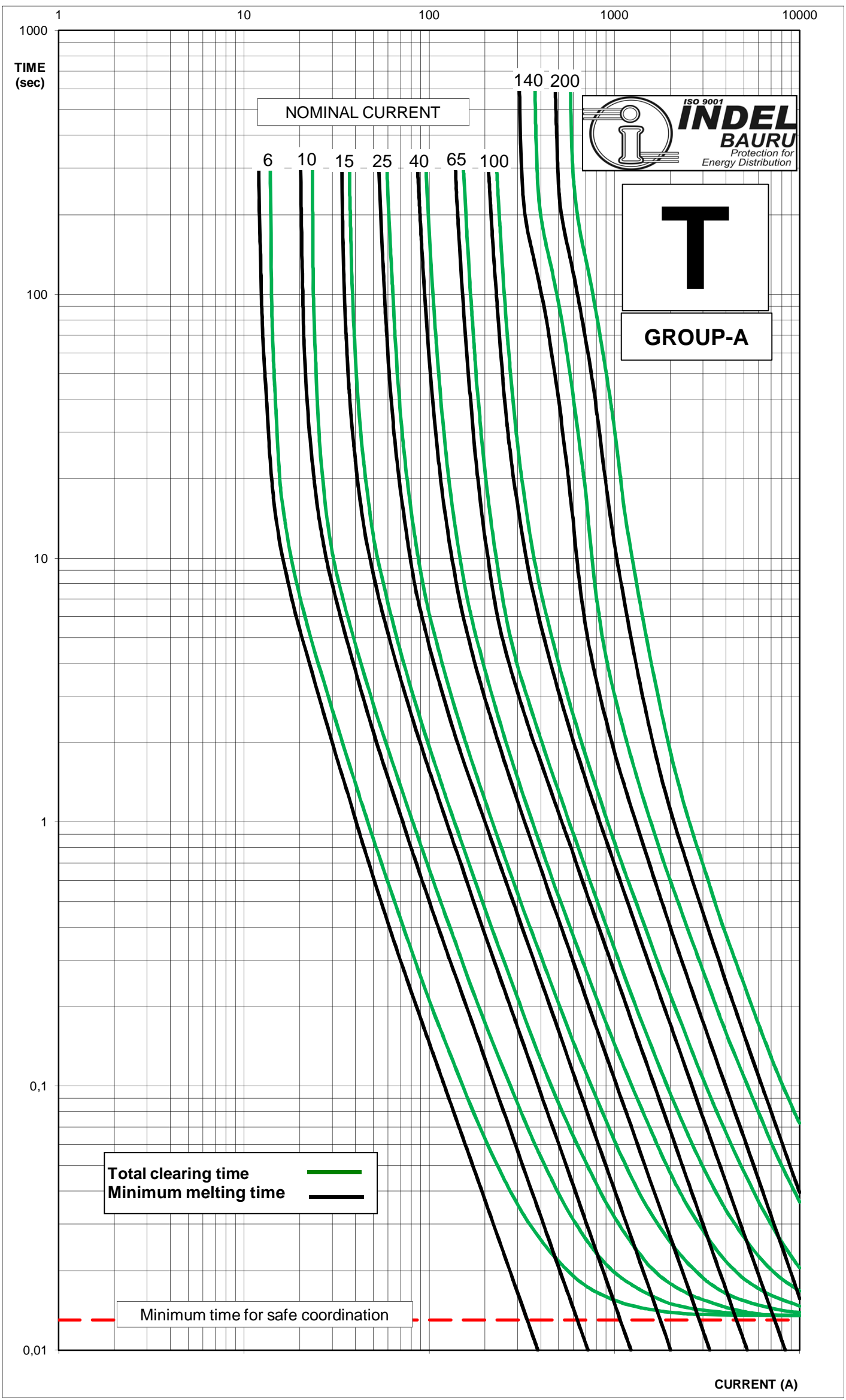
CHARACTERISTICS CURVES FUSION TIME x CURRENT TYPE "T" - COMPLY WITH STANDARD ANSI C37.42-1996 DATE: 09/02
